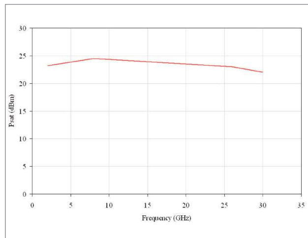
Figure 11. Saturated output power
